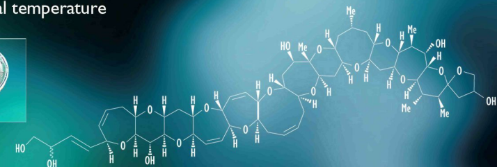
Ciguatoxin (CTX-1B)
