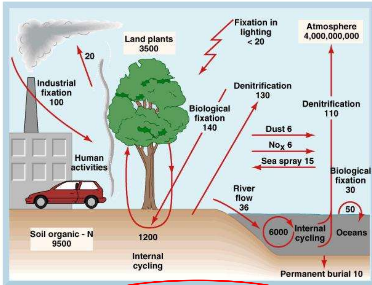
The global nitrogen cycle. Pools (□) and annual (→) flux in 10^{12} \text{g N}_2 . Note that the industrial fixation of nitrogen is nearly equal to the global biological fixation. (SOURCE: Data from Söderlund, and T. Rosswall, 1982, O. Hutzinger (ed.), The Handbook of Environmental Chemistry , Vol 1, Pt. B., Springer-Verlag New York, Inc., New York).
