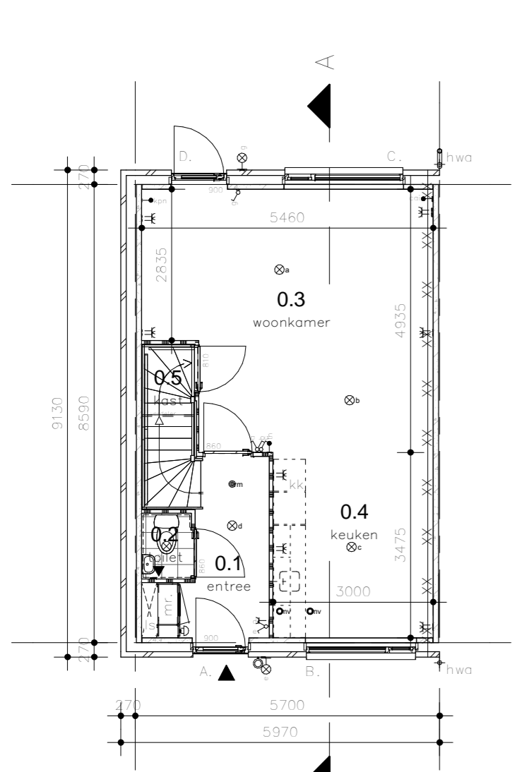
Begane grond (0.000+)
